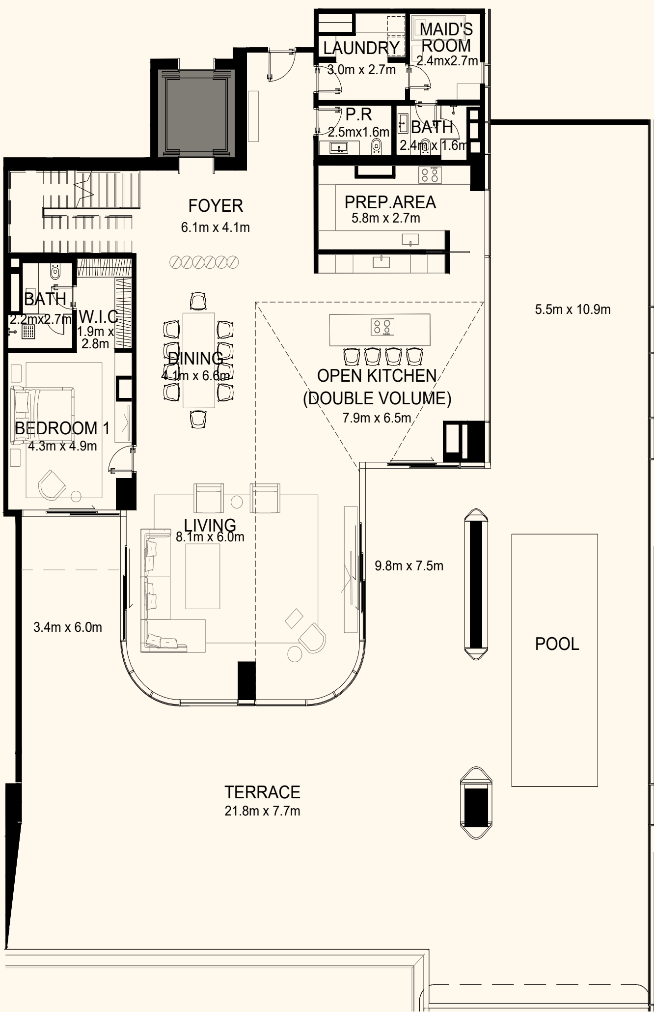
Lower Level
