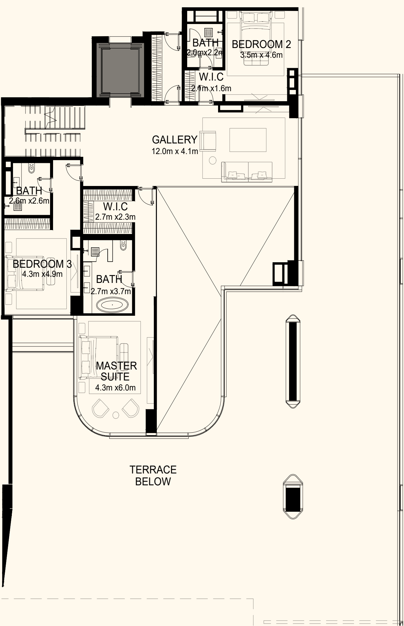
Upper Level
