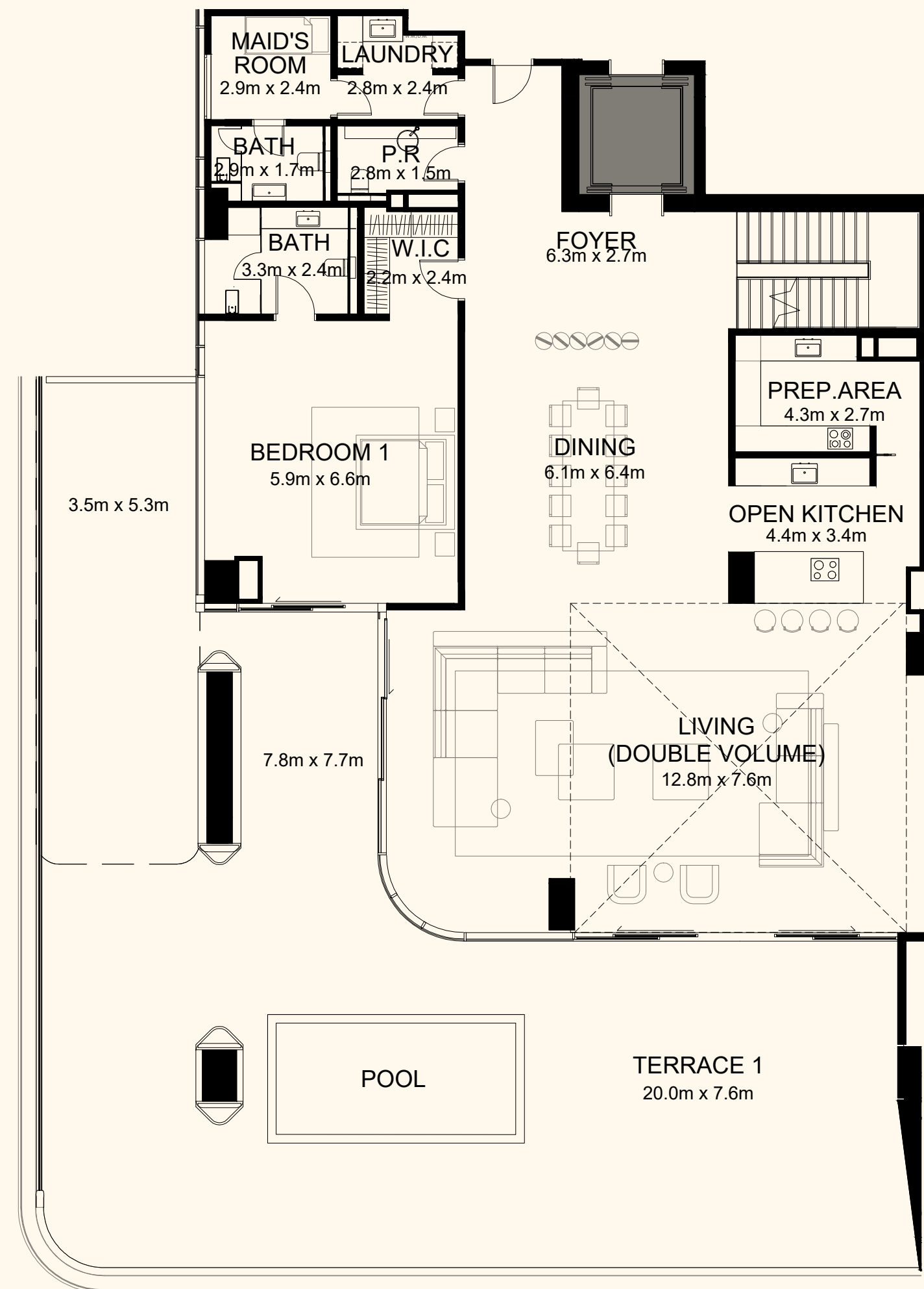
Lower Level
